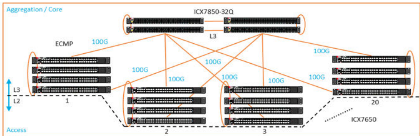
FIGURE 1 Routed Access
