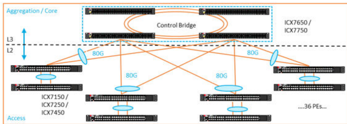
FIGURE 7 Campus Fabric
